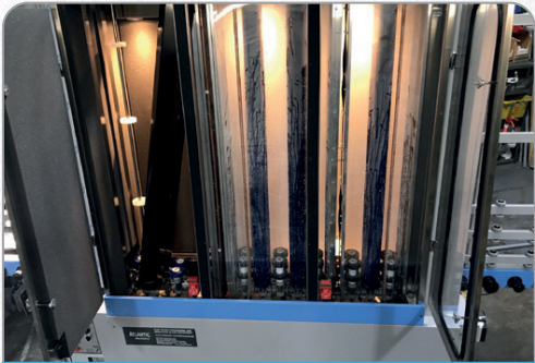
ATL-V-15-6B right to left running with covers open showing layout and easy access
